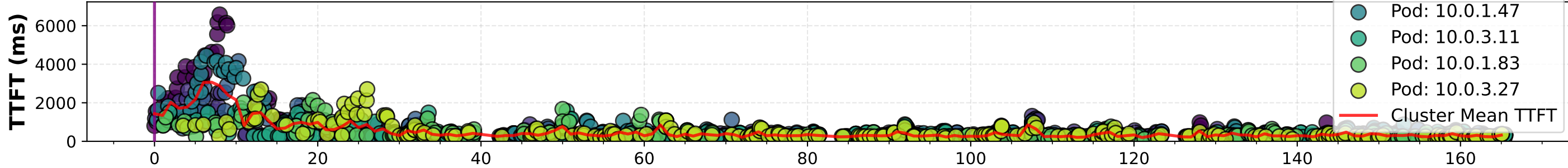
Time to First Token (TTFT) for Each Request
