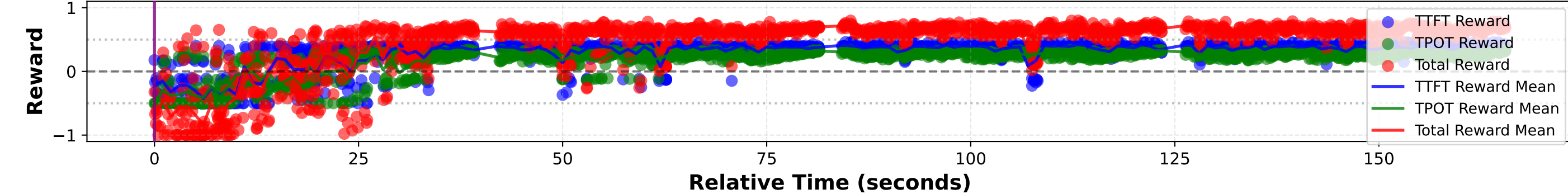
Reward Time Series (SLO: TTFT≤1000ms, TPOT≤50ms)
