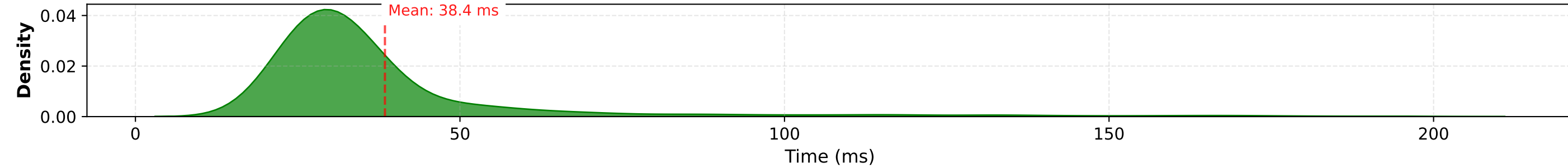
TPOT Distribution
