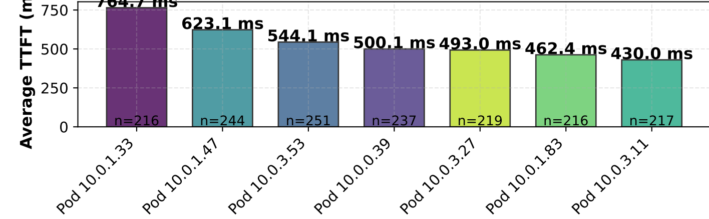
TTFT Distribution
