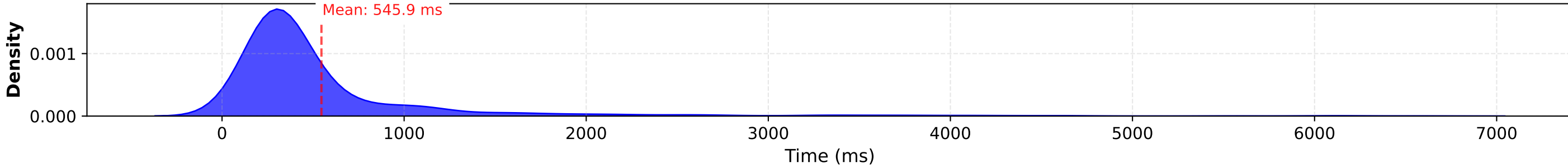
TTFT Distribution
